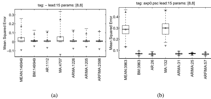
Fig. 5. Performance of 8 parameter host load prediction models for 15 second ahead predictions: (a) All traces, (b) Moderately loaded interactive host.
