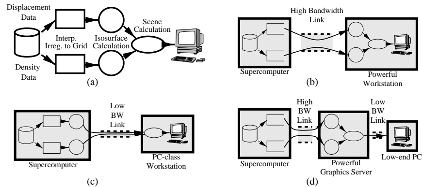
Fig. 1. QuakeViz Application. (a) Stages of the Quake visualization toolchain. Different placements of toolchain tasks corresponding to different resource situations: (b) A high performance network and workstation are available for the visualization. (c) A low-bandwidth network and PC with a 3D graphics accelerator are used. (d) A low-end PC is used as a framebuffer displaying the result of a completely remote visualization process.
