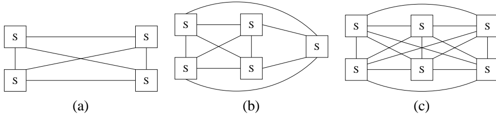
Figure 13. Examples of switch cliques with 4, 5 and 6 nodes.
