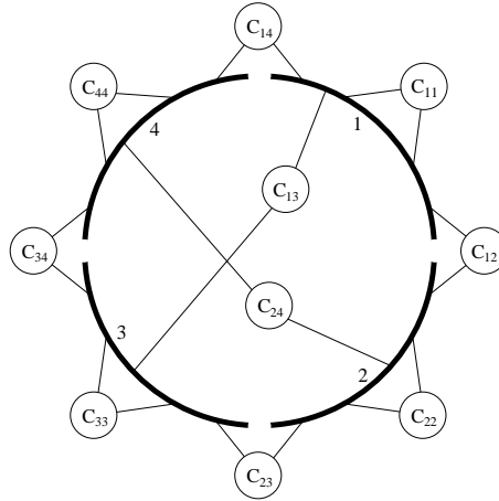
Figure 9. Node types after the introduction of 4 faults in the ring. All nodes are classified by the switch segments they are connected to.
