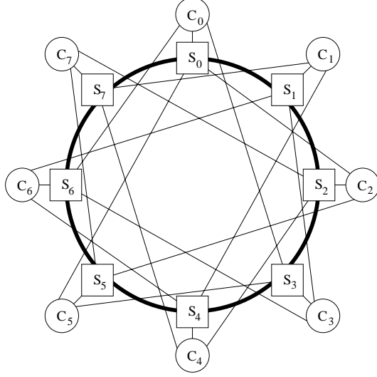
Figure 11. Generalized diameters construction for d_c = 3 and n = 8 .
