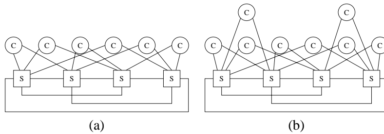
Figure 14. Examples of homogeneous clique-based systems with (a) 4 switches and 6 nodes, (b) 4 switches and 8 nodes.
