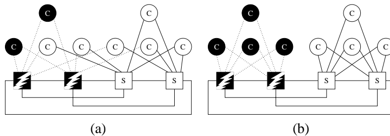
Figure 15. Examples of faults and the related node loss. In (b) the upper bound is achieved.
