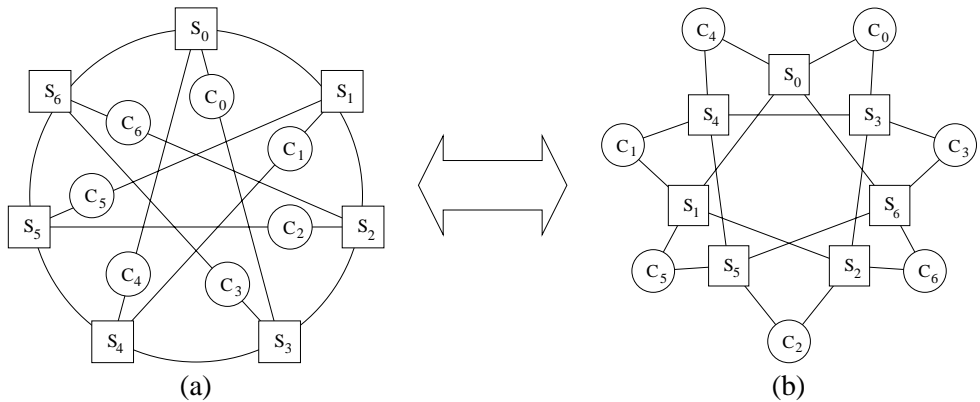
Figure 12. (a) Normal construction layout. (b) A new layout for the same graph with short node-to-switch links.
