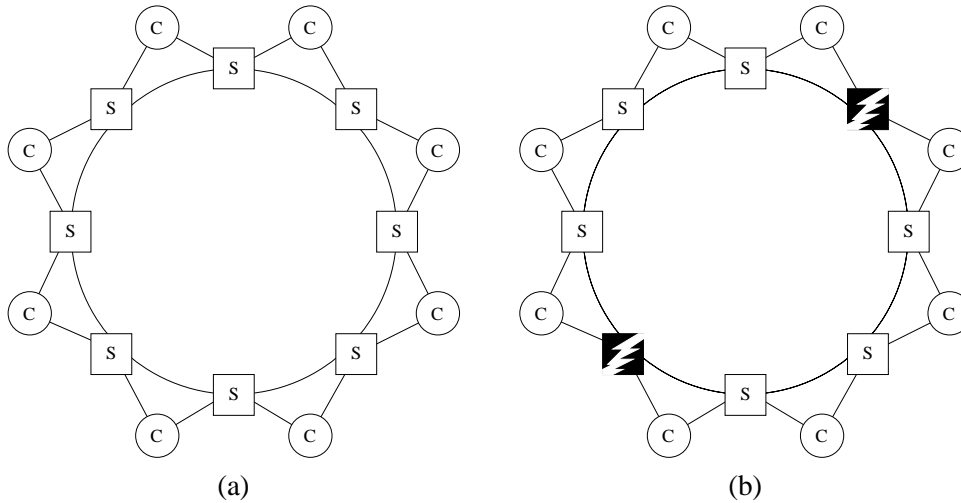
Figure 7. (a) A naïve approach, d_c = 2 . (b) Notice that it is easily partitioned with two switch failures.
