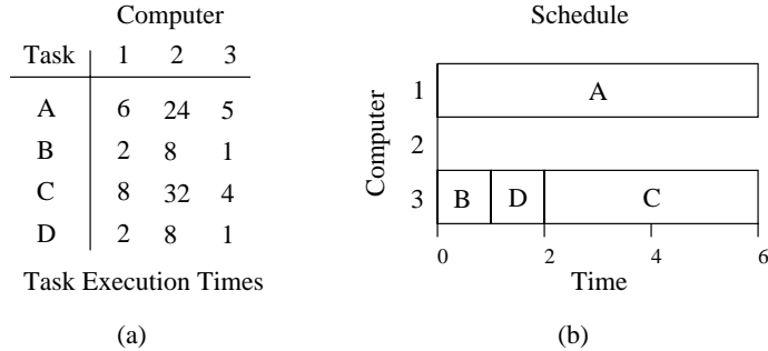
Figure 1: An example where neither load balancing nor user directed assignments are the best scheduling strategies for a metacomputer. Table (a) gives the execution times of each task of a set of jobs on each machine. A Gantt chart of the schedule that minimizes the schedule length is shown in (b).
